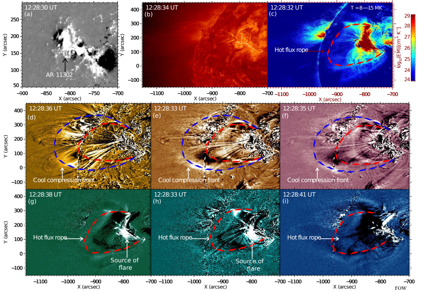
Figure 8. Multi-wavelength view of magnetic flux-rope as seen in different wavebands of SDO/AIA. Top row (panels a–c): The hot flux-rope formed above an active region, AR 11302, as shown by SDO/HMI line-of-sight magnetograms (panel a). The SDO/AIA 304 Å image depicts the absence of flux-rope/eruption (panel b). The panel (c) indicates the presence of a hot flux-rope (8–15 MK) in the DEM map. Middle row (panels d–f): It shows the distinct feature of the magnetic flux-rope in its eruptive phase. The cyan dotted lines show the cool compression front, followed by the dark cavity region of the flux-rope, which best appears at coronal temperature (0.6–2 MK) in AIA 171 Å, 193 Å, and 211 Å wavebands. Bottom row (panels g–i): The hot channel of the flux-rope has been shown via dotted red lines in the hotter wavebands of AIA (2.5–10 MK, i.e., 94 Å, 131 Å, and 335 Å). It should be noted that cool coronal images (middle panel) show the very faint signature of this hot channel of the flux-rope.
