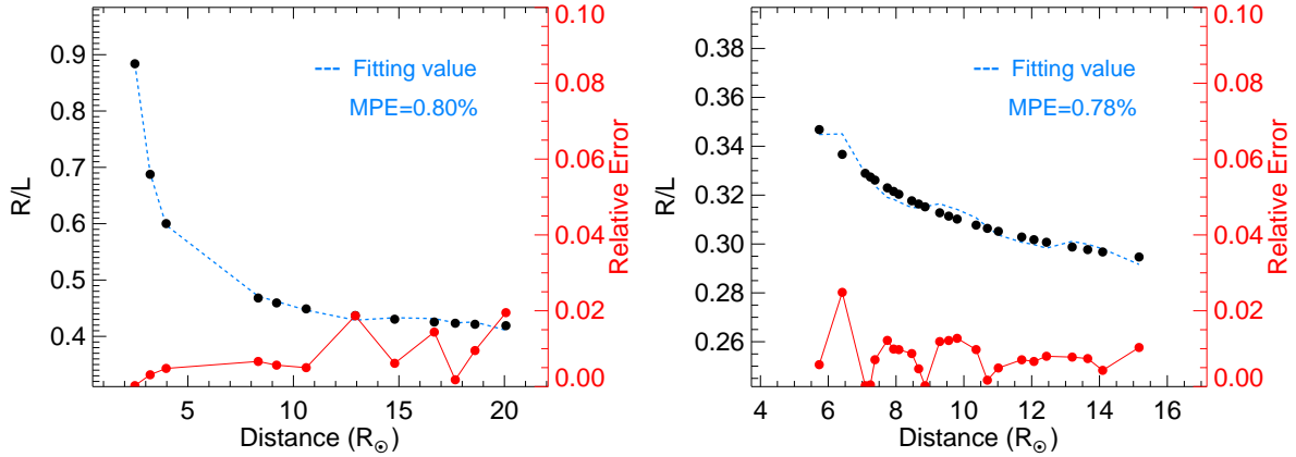
Figure 4. The profile of R/L for CME1 and CME2 from the measurements (black; left-hand side of Equation 1), the model-fitted result for this parameter (blue; right-hand side of Equation 1), and the relative error (red) are shown. (MPE: Mean Percentage Error)
