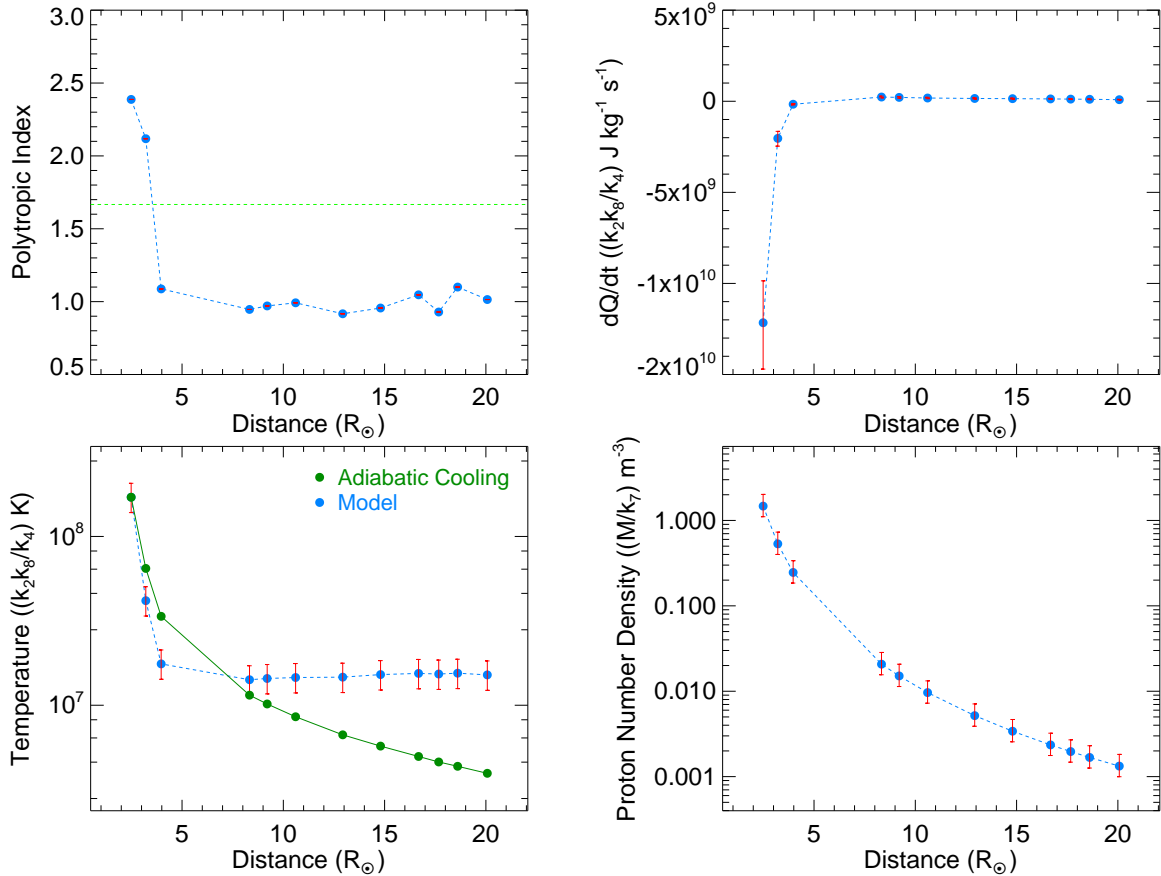
Figure 5. For the CME1: Variation of the polytropic index ( \Gamma ), average heating rate ( dQ/dt ), average temperature ( \bar{T} ), and average proton number density ( \bar{n}_p ) of the CME with the heliocentric distance of the CME's leading edge ( h ) is shown in the top-left, top-right, bottom-left and bottom right, respectively. The red vertical lines at each data point show the error bars derived by considering an error of 10% in measurements of the flux-rope's leading edge height ( h ).
