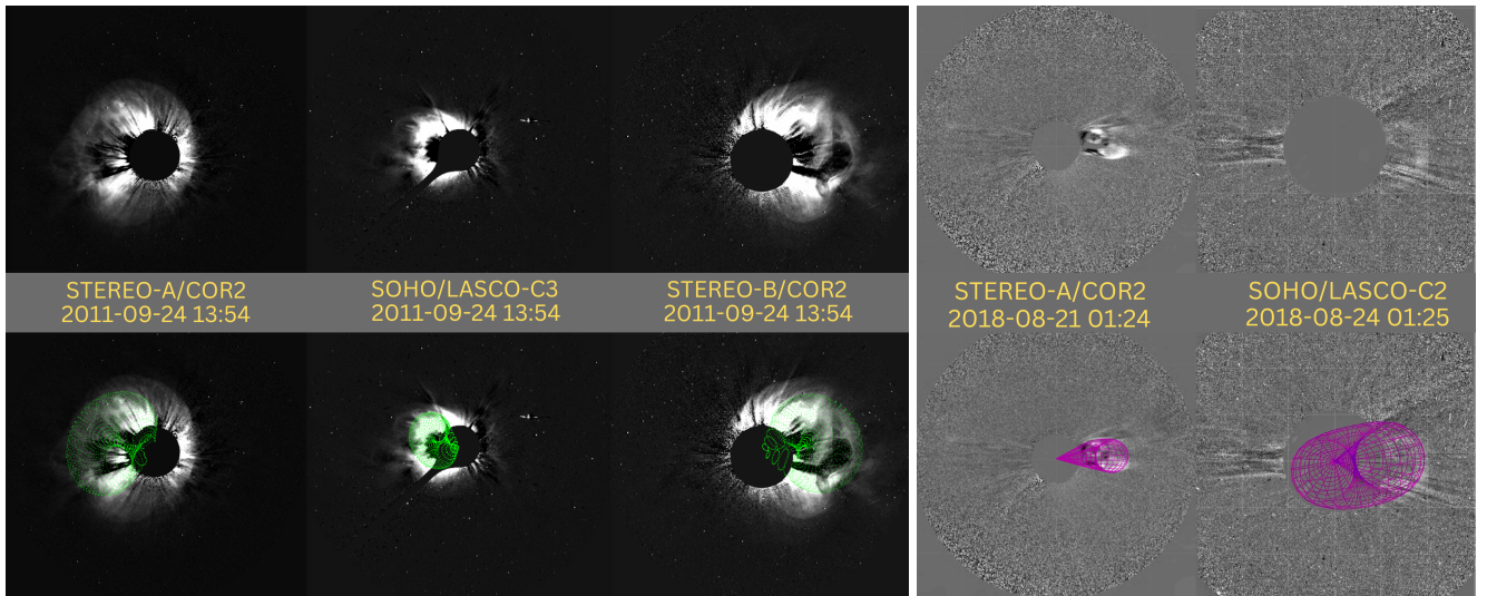
Figure 2. The GCS model fitted wireframe in green and pink overlay on the contemporaneous coronagraphic images of the CME1 shown in left (left: STEREO-A/COR2, centre: LASCO-C3, right: STEREO-B/COR2) and for CME2 shown in the right (left: STEREO-A/COR2, right: LASCO-C2), respectively.
