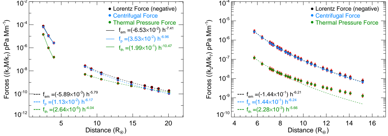
Figure 7. The FRIS model-derived average internal forces, such as Lorentz force, Thermal pressure force, and Centrifugal force, that is responsible for the radial expansion of the flux-rope of CME1 (left) and CME2 (right). The red vertical lines at each data point show the error bars derived by considering an error of 10% in measurements of the leading edge height of the flux-rope ( h ). The solid and dash lines show the power-law fitted values for the model-derived internal forces.
