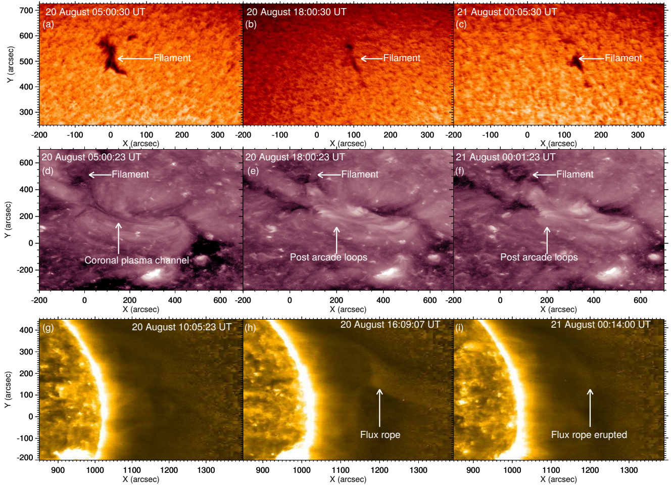
Figure 9. Top row (panels a–c): The sequence of images of GONG/H \alpha shows the gradual eruption of a quiescent filament on 2018 August 20. It is associated with an elongated filament channel containing no cool component but a hot plasma channel. Middle row (panels d–f): Temporal evolution of coronal plasma channel (hot filament channel) lying between two coronal holes as observed by SDO/AIA 211 Å. Bottom row (panels g–i): The formation of flux-rope and its eruption lying over the coronal plasma channel is shown in STEREO-A/EUVI 171 Å on 2018 August 20.
