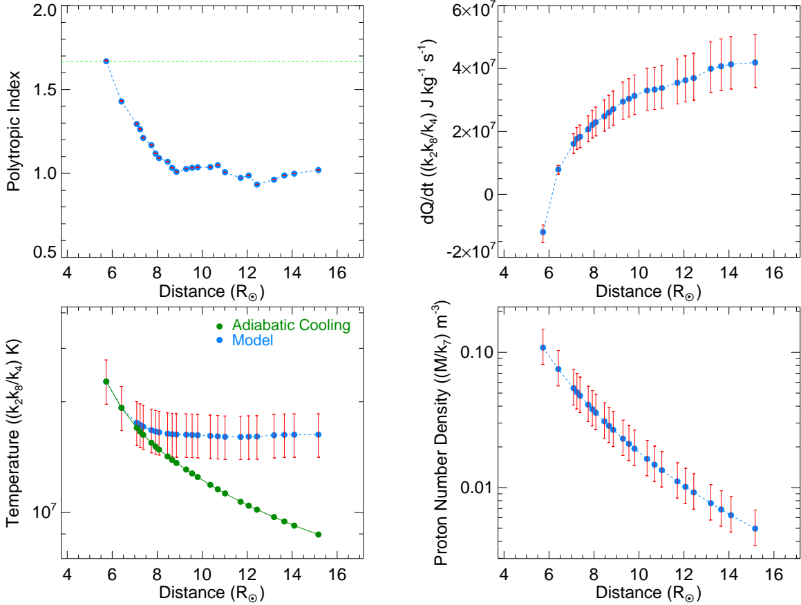
Figure 6. For the CME2: Variation of the Polytropic index ( \Gamma ), average heating rate ( dQ/dt ), average temperature ( \bar{T} ), and average proton number density ( \bar{n}_p ) of the CME with the heliocentric distance of the CME’s leading edge ( h ) is shown in the top-left, top-right, bottom-left and bottom right, respectively. The red vertical lines at each data point show the error bars derived by considering an error of 10% in measurements of the flux-rope’s leading edge height ( h ).
