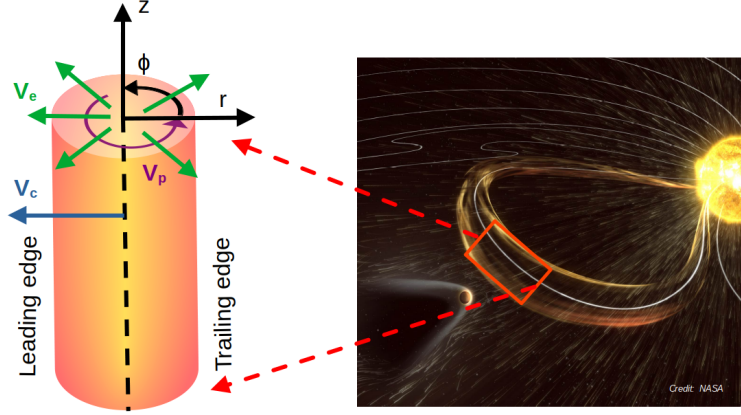
Figure 1. Schematic of a flux-rope CME in the cylindrical coordinate system (i.e r, \phi, z ) showing the propagation speed ( v_c ) of the axis of the flux-rope, expansion speed ( v_e ), and poloidal speed ( v_p ).
